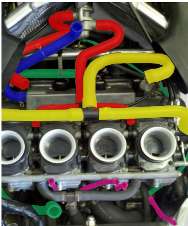
1999 CBR600 F4 49-STATE RED SECONDARY AIR SYSTEM PINK VACUUM TUBES YELLOW VACUUM CHAMBER VENT HOSES BLUE CRANKCASE BREATHER HOSE GREEN PAIR VALVE HOSES BY CJARDINE FOR CBRFORUM
